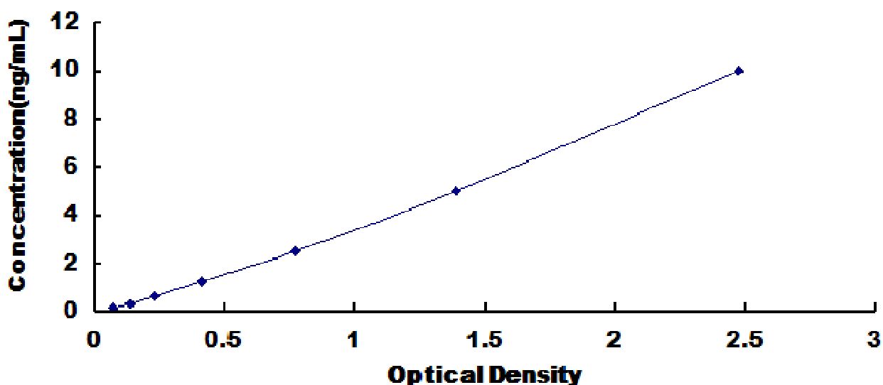
Typical Standard Curve for ADORA1, Rat ELISA.
