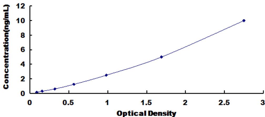
Typical Standard Curve for APC, Rat ELISA.
