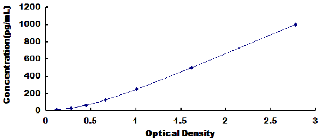
Typical Standard Curve for ADAM8, Mouse ELISA.
