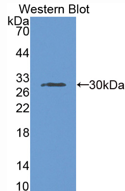
Used in Western Blot, Sample: Recombinant RNPEP, Human
