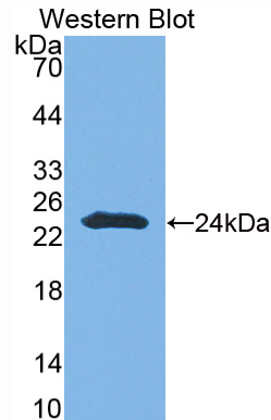
Used in Western Blot, Sample: Recombinant CNTNAP4, Human
