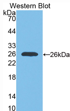
Used in Western Blot, Sample: Recombinant IGF1R, Human
