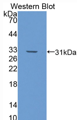
Used in Western Blot, Sample: Recombinant GSTt1, Mouse
