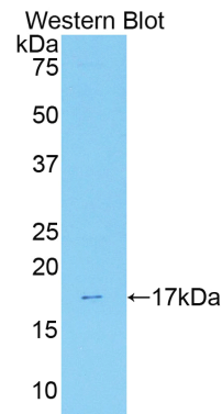
Sample: Recombinant ANXA3, Mouse
