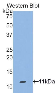
Sample: Recombinant SEPW1, Human
