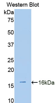
Used in Western Blot ,Sample: Recombinant ADAMTS1,Mouse
