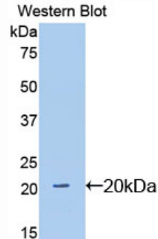
Used in Western Blot ,Sample: Recombinant SIGLEC12,Mouse
